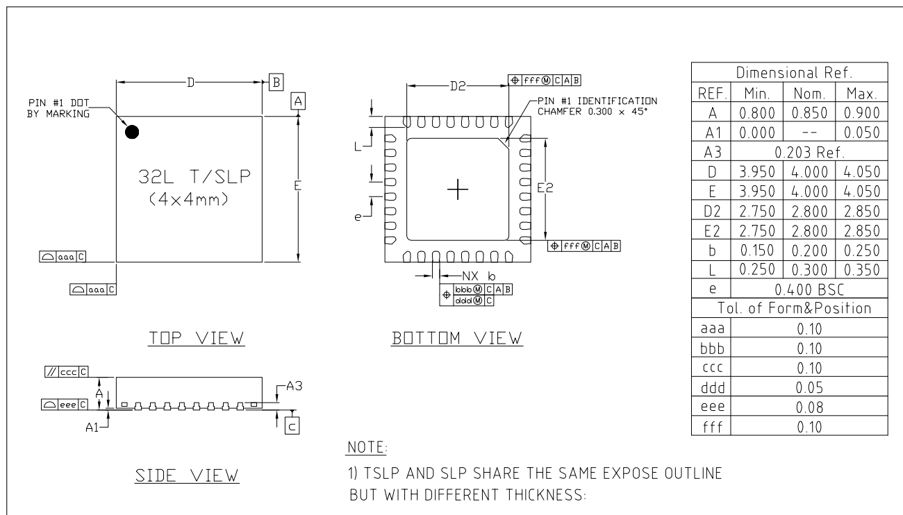
Figure 7-1. QFN32 (4×4 mm) Package
